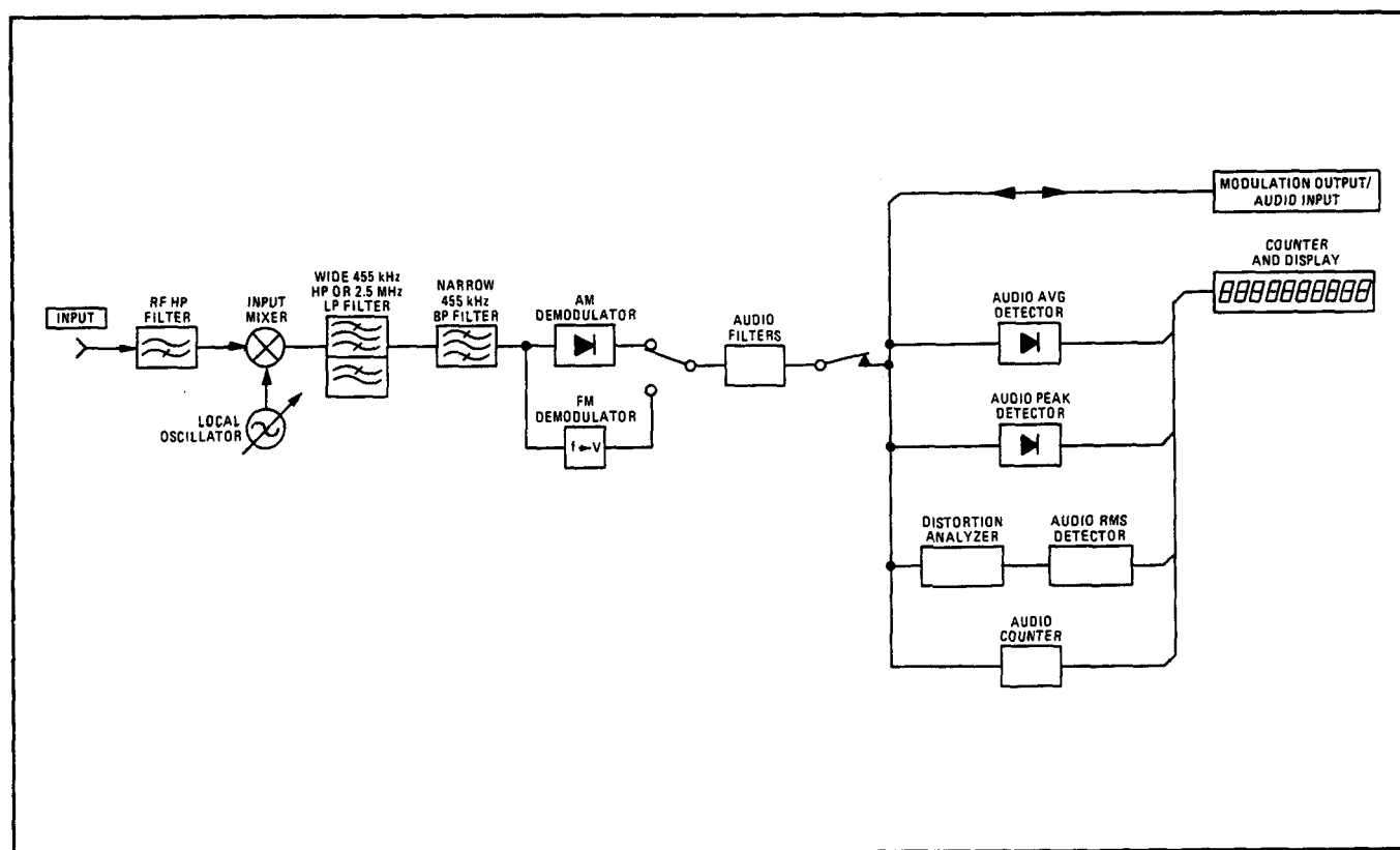
Audio Filters Block Diagram
