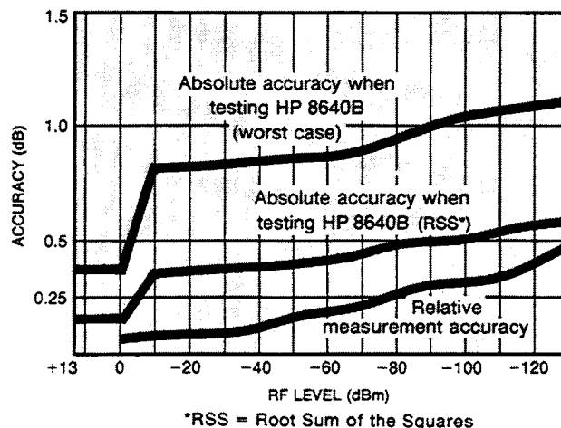
Graph 4-1. Tuned RF Level Measurement Accuracy.
