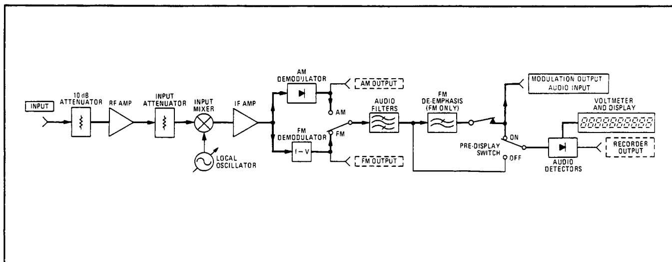
Modulation Output/Audio Input Block Diagram
