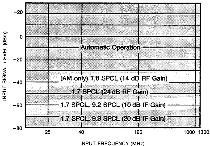
Diagram 3-1. Typical Modulation and Audio Measurement Ranges
