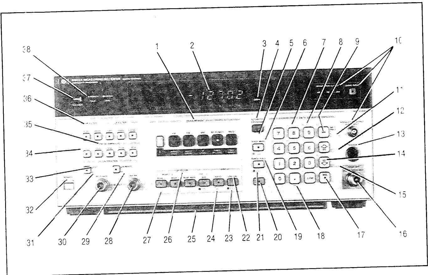
Figure 3-1. Front-Panel Features
