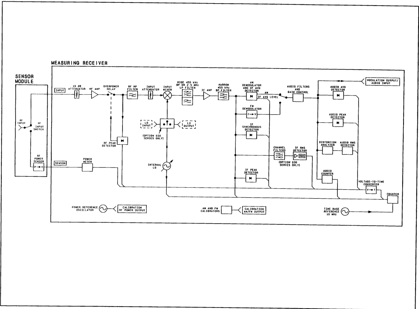
Figure 1-2. HP 8902A Measuring Receiver Simplified Block Diagram
