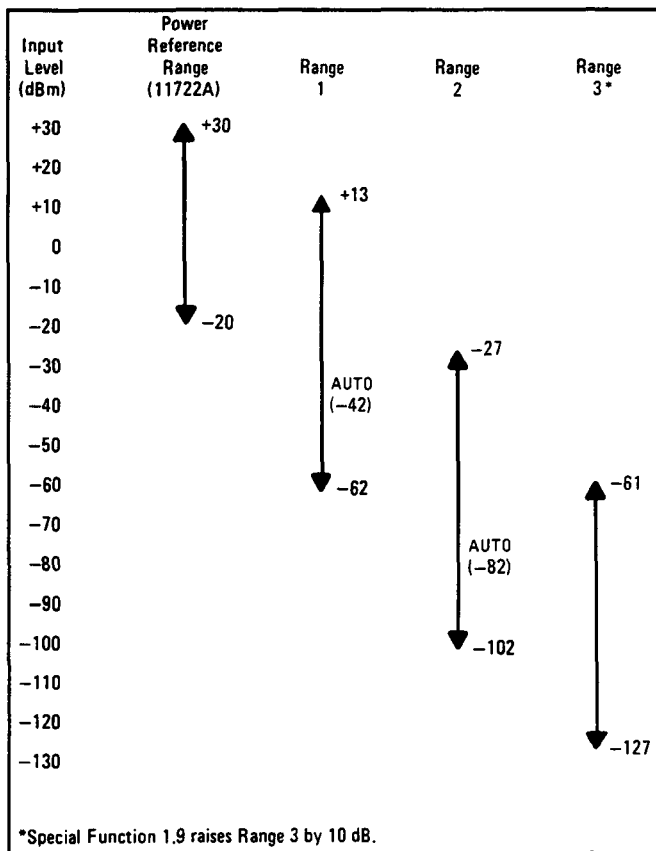
Synchronous Tuned RF Level Ranges
