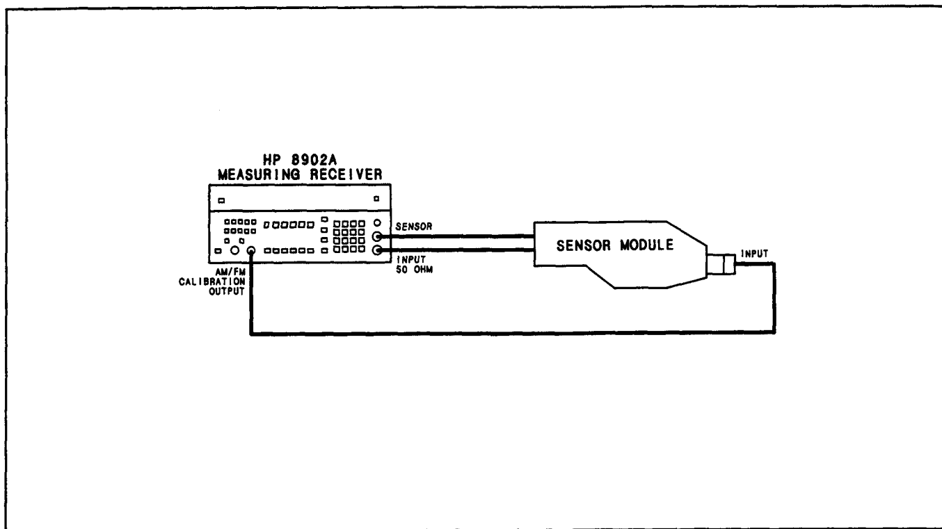
Figure 3-8. AM and FM Calibration Check Setup
