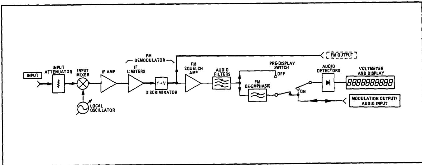
FM Output Block Diagram
