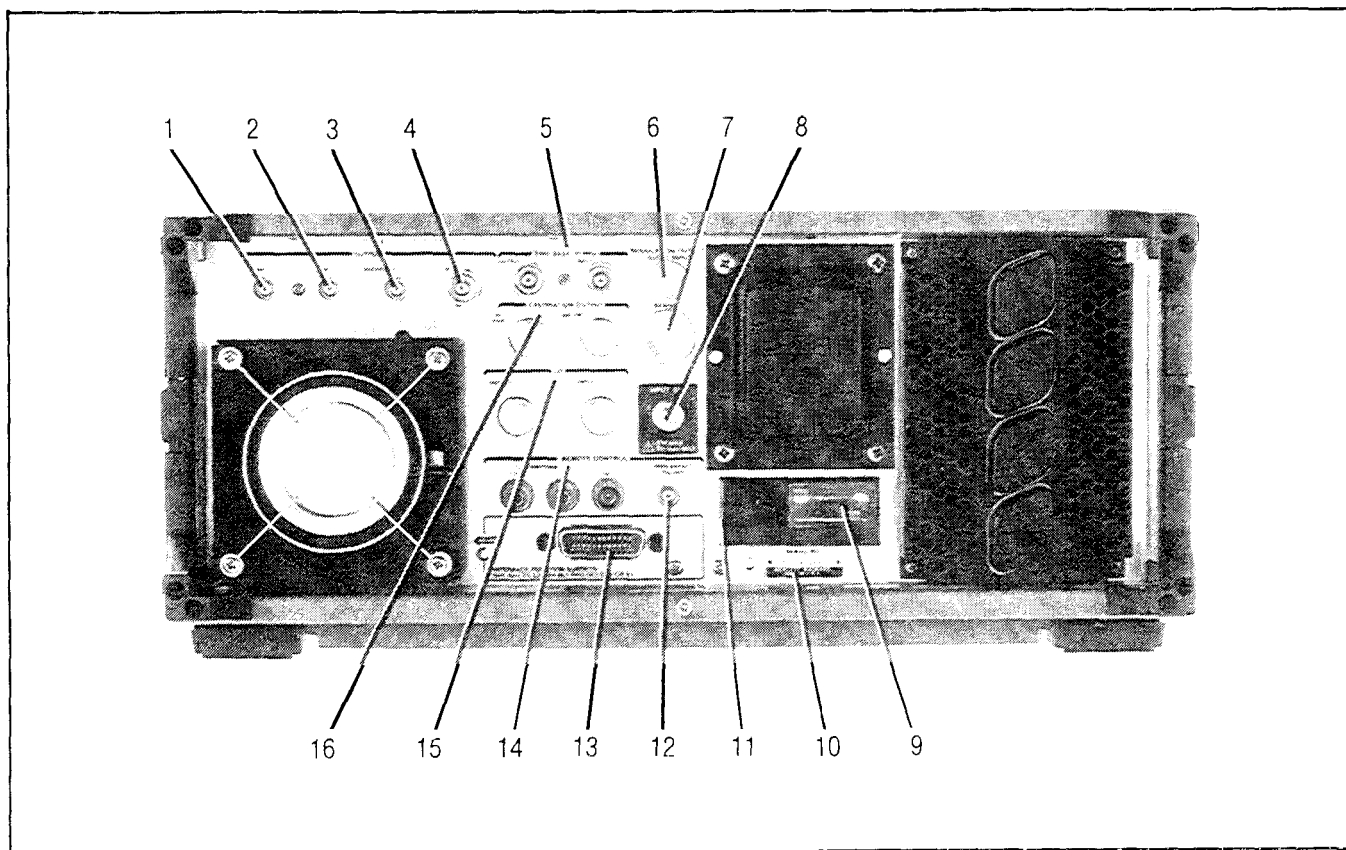
Figure 3-2. Rear-Panel Features
